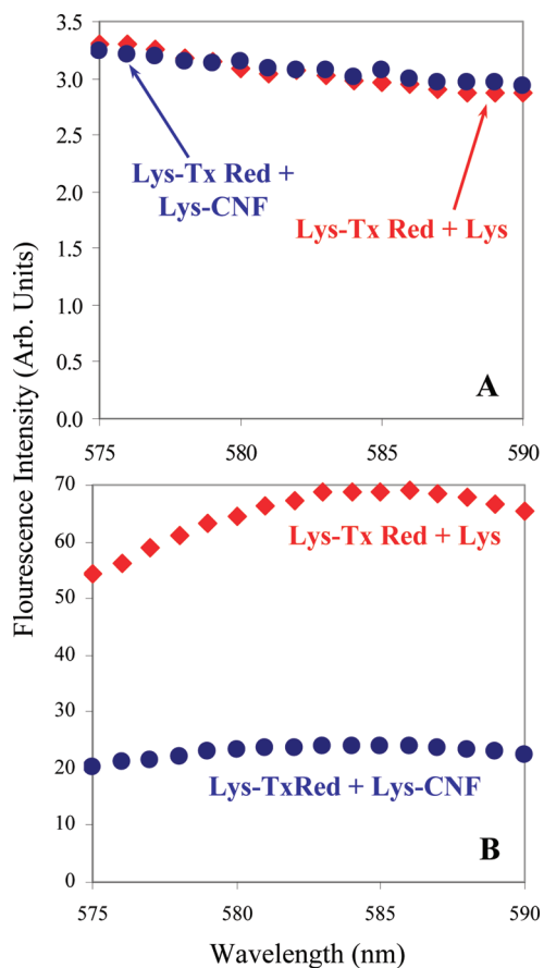
Figure 3. Fluorescence spectra for FRET labeled Lys with surface coverages of 0.016 \mu\text{mol}/\text{m}^2 (A) and 0.305 \mu\text{mol}/\text{m}^2 (B). The spectra show no quenching at low protein loading and substantial quenching at high surface coverage.
