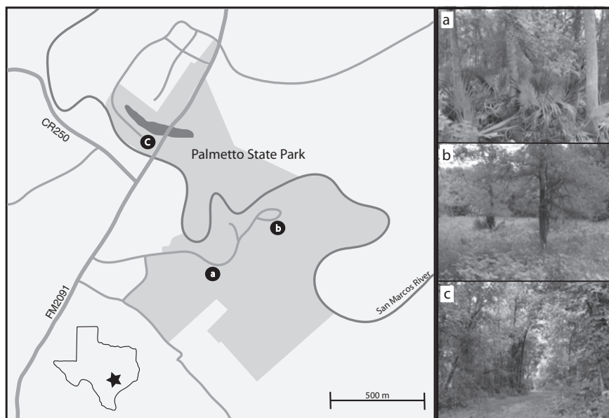
Figure 1 Study plots within Palmetto State Park, Gonzales, Texas. The star on the small map of Texas (bottom left) indicates the location of the park within the state.
