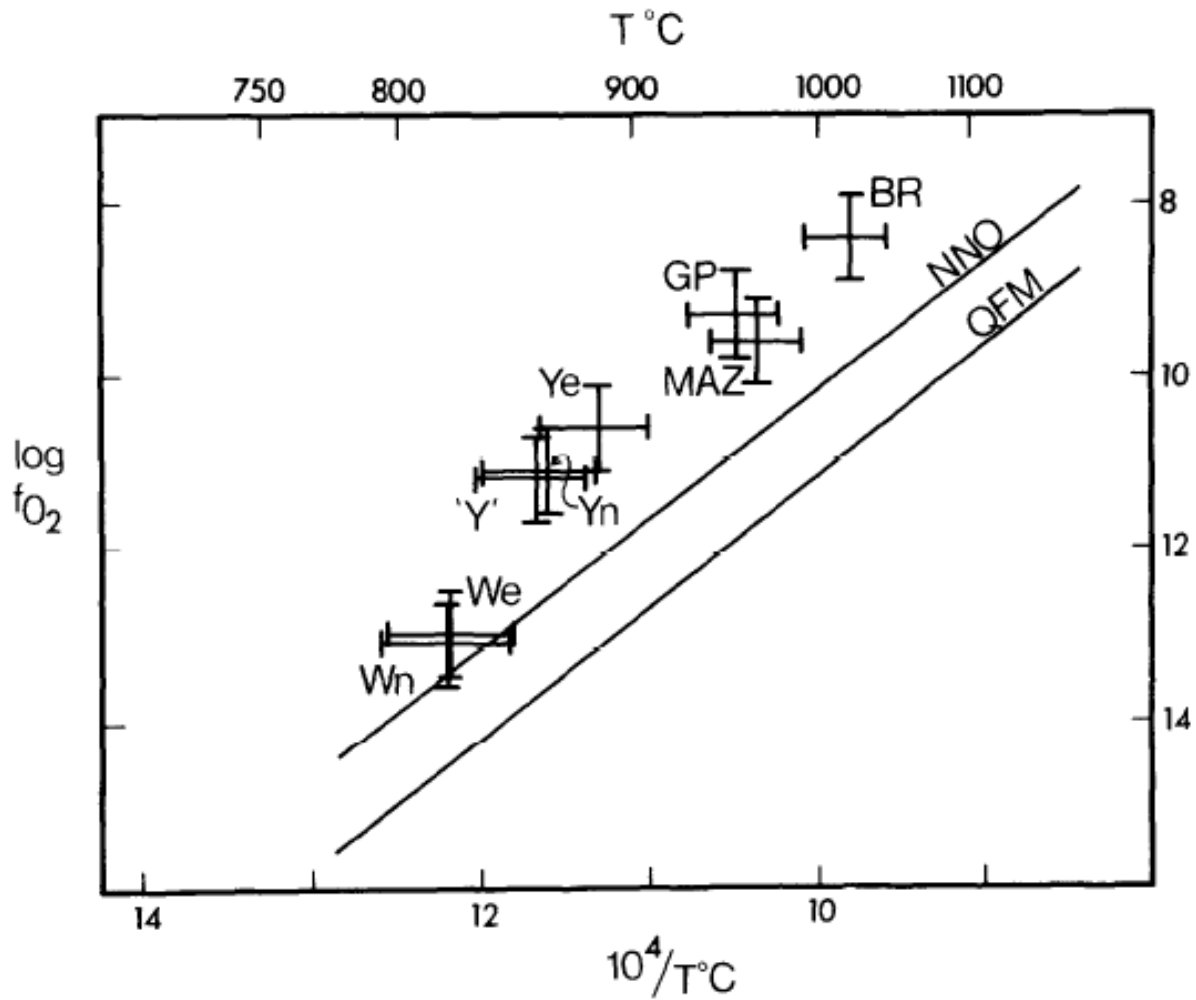
FIG. 9. Temperature vs -\log f_{O_2} for various Pacific Northwest tephras. The average values are plotted with error bars indicating a range of \pm 25^{\circ}C and \pm 0.5 log unit. "Y" represents T-f_{O_2} values derived using previously published analyses of Fe-Ti oxides attributed to tephra set Y; other abbreviations as in Figure 1.
